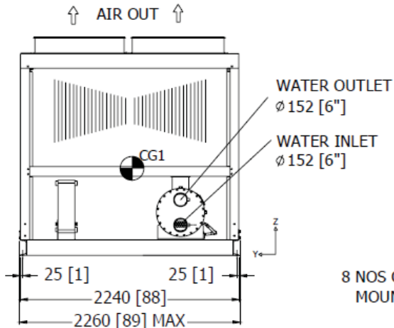
LEFT VIEW
